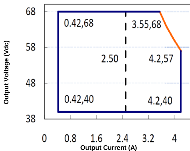
Figure 3: Typical V-I Characteristic Curve (LTA240X-068C)
