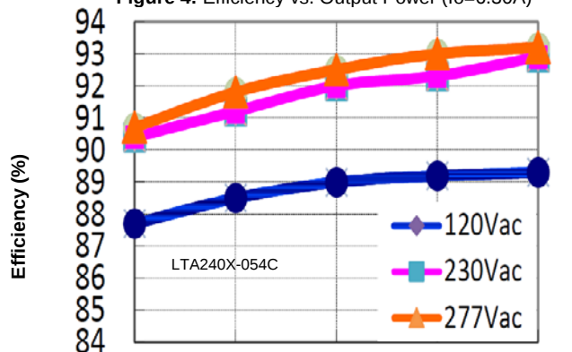
Figure 4: Efficiency vs. Output Power ( I_o=6.30A )
