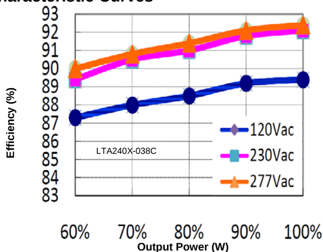
Figure 4: Efficiency vs. Output Power ( I_o=6.30A )
