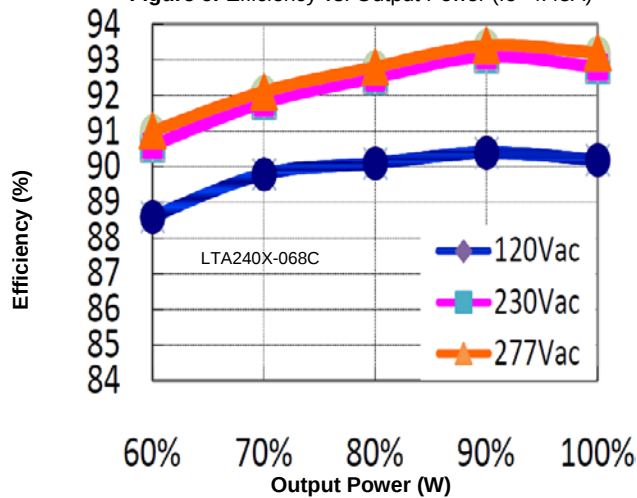
Figure 8: Efficiency vs. Output Power ( I_o=3.55A )
