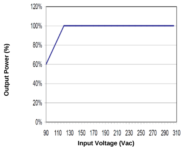
Figure 11: Output Power vs. Input Voltage
