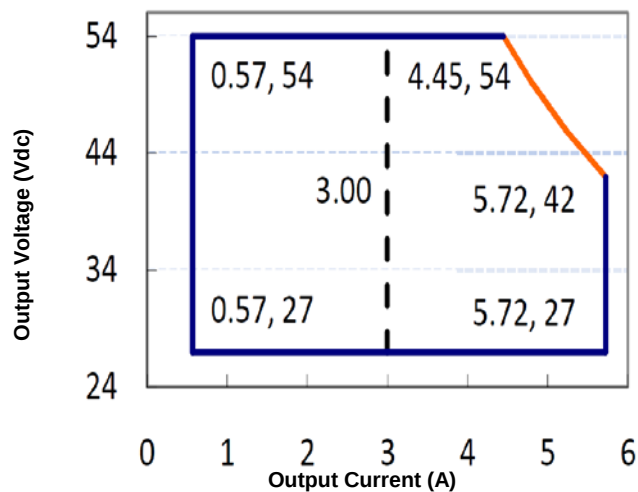
Figure 2: Typical V-I Characteristic Curve (LTA240X-054C)
