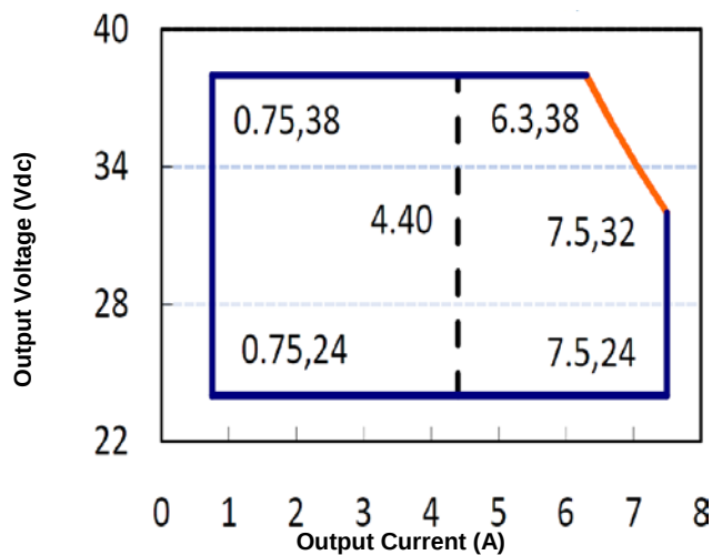
Figure 1: Typical V-I Characteristic Curve (LTA240X-038C)
